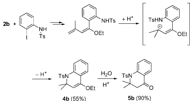
Scheme 4. Direct synthesis of cyclic derivative 4b through the formation of a stable carbocation.
